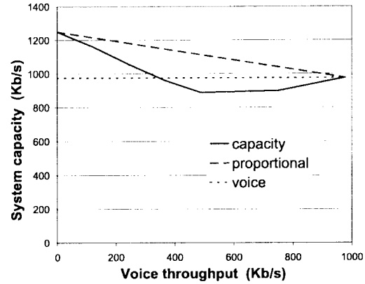
Fig. 1. System capacity as function of the voice throughput.
