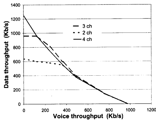
Fig. 2. Maximum throughput reached by data as function of the voice throughput, when using 2, 3, and 4 channels with SF = 8 and R = 1/2 .
