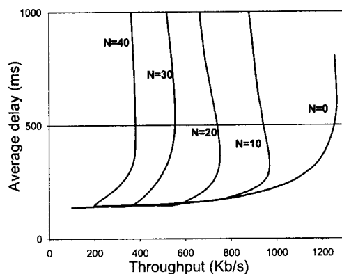
Fig. 3. Delay-throughput curve for data traffic when using 4 channels with SF = 8 and R = 1/2 , with a different number of voice calls.
